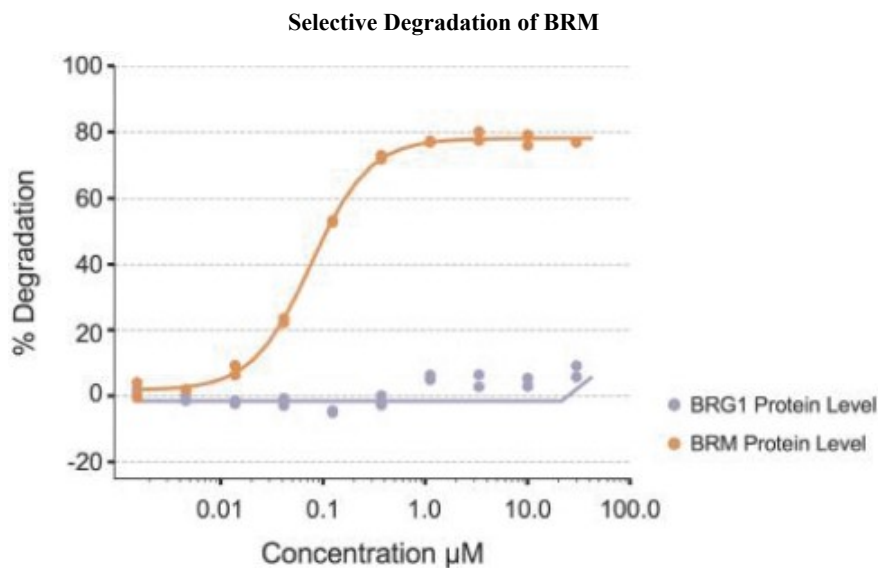
Figure 9. Selective BRM degrading molecules led to the degradation of over 75 percent of BRM while leaving the levels of BRG1 virtually unchanged.
